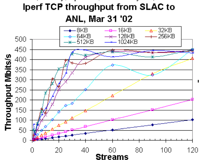
Figure 4: Ten second iperf TCP throughputs from SLAC to ANL
