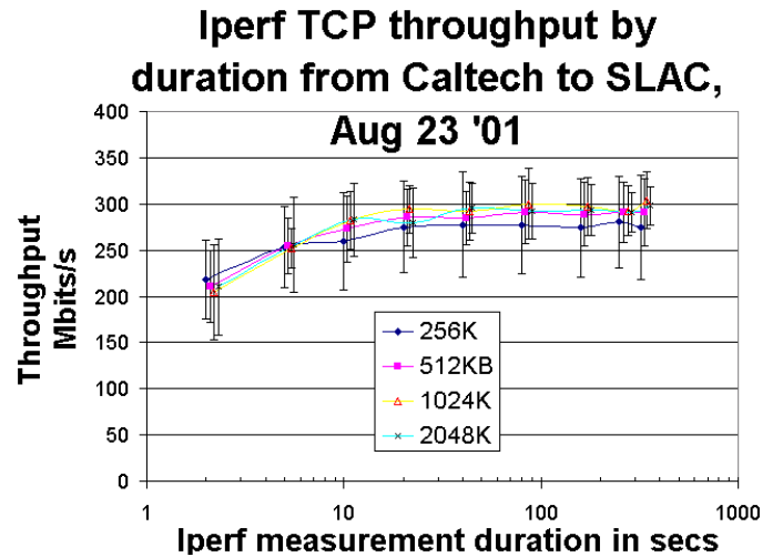
Figure 2: Iperf TCP throughput by measurement duration from SLAC to Caltech, Aug 23 2001
